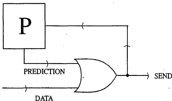
Fig. 4.5 A Predictive Encoder
