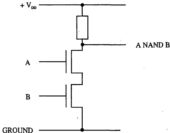
Fig. 7.18 The NAND Gate Realized by MOSFETS
