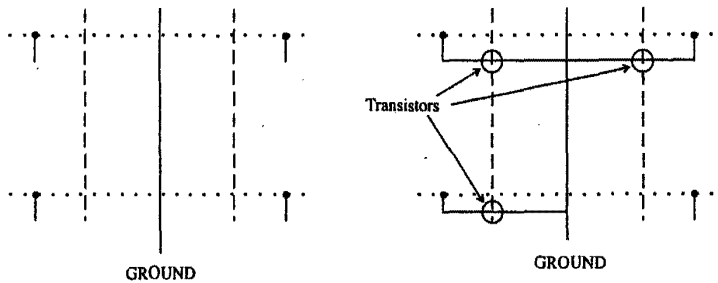
Fig. 7.65 A Generic AND plane and the Amended Form
