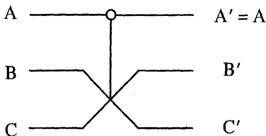
Fig. 2.23 The Fredkin Gate: A Controlled Exchange
