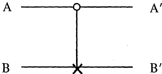
Fig. 2.20 The CN Gate
