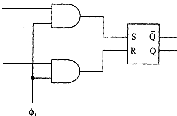
Fig. 2.30 A Clocked RS Flip-Flop
