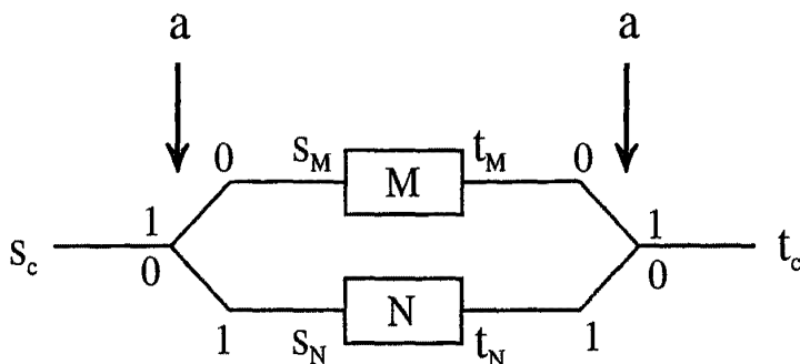
Fig. 6.12 Conditional: if a = 1 then M , else N
