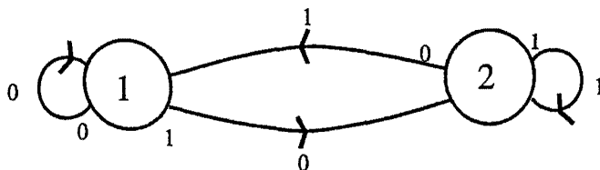
Fig. 3.4 A Delay Machine
