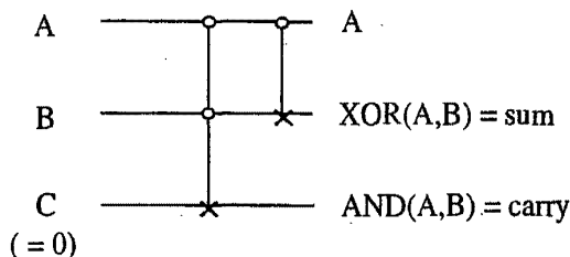
Fig. 5.25 A Two-bit Adder From Reversible Gates
