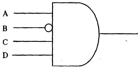
Fig. 2.15 A Simple Decoder
