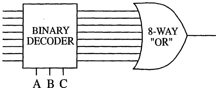
Fig. 2.17 The Multiplexer
