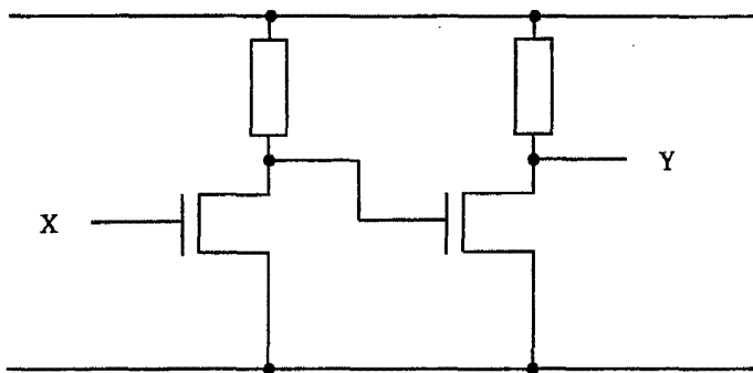
Fig. 7.20 "Follower" Circuit
