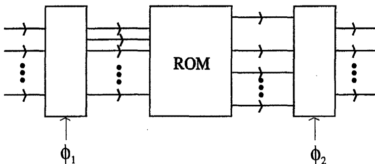
Fig. 7.62 Clocked ROM Control System
