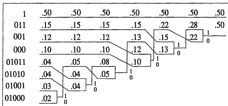
Fig. 4.3 Huffman Coding Tree
