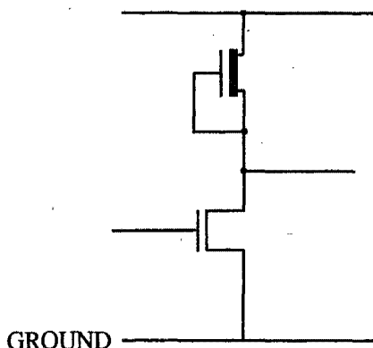
Fig. 7.19 nMOS Inverter with MOSFET Resistance
