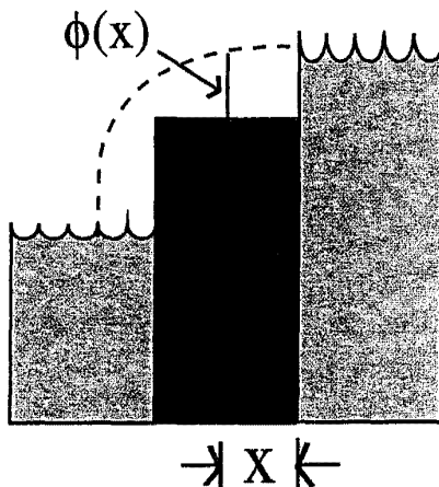
Fig. 7.11 Fluid Analogy for the Case of Saturation of the MOSFET
