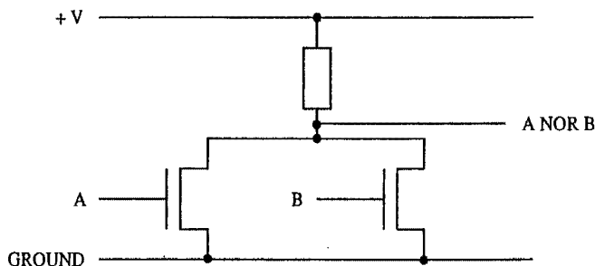
Fig. 2.14 A Transistor NOR Gate
