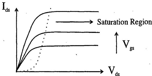
Fig. 7.12 Current-Voltage Variations for MOSFET
