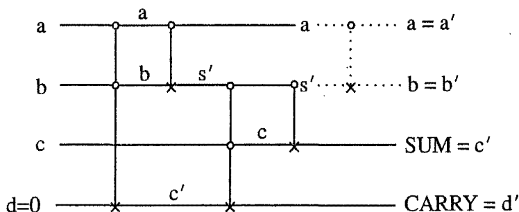
Fig. 6.5 A Full Adder
