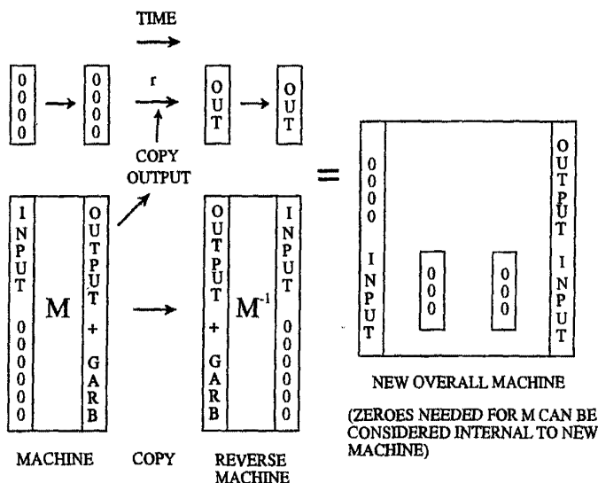
Fig. 6.6 Clearing Garbage
