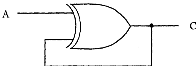
Fig. 2.27 A Plausible (but Non-Workable) Memory Device
