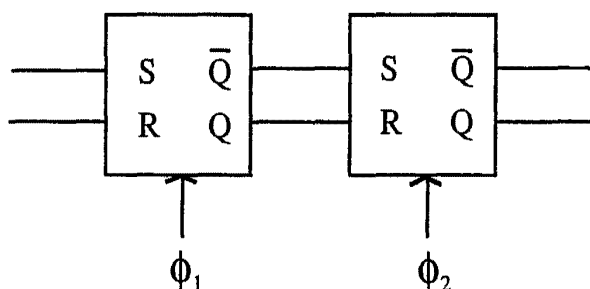
Fig. 2.32 The Master-Slave Flip-Flop
