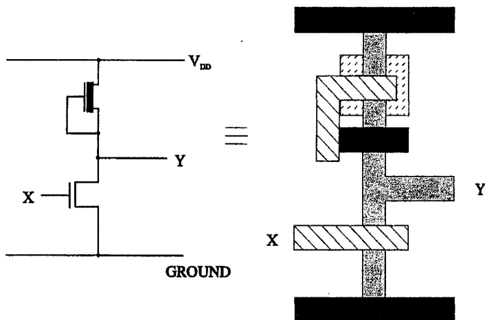
Fig. 7.51 The Full Inverter
