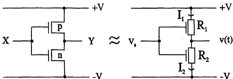
Fig. 7.34 Simplified Model of a CMOS Inverter
