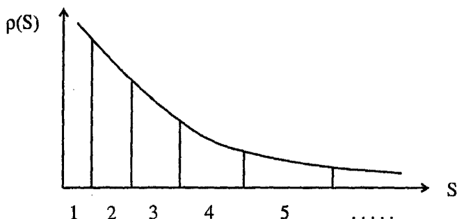
Fig. 4.7 Division of \rho(S) into Equal Volume Bins
