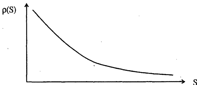
Fig. 4.6 A Sample Probability Distribution for a Physical Variable
