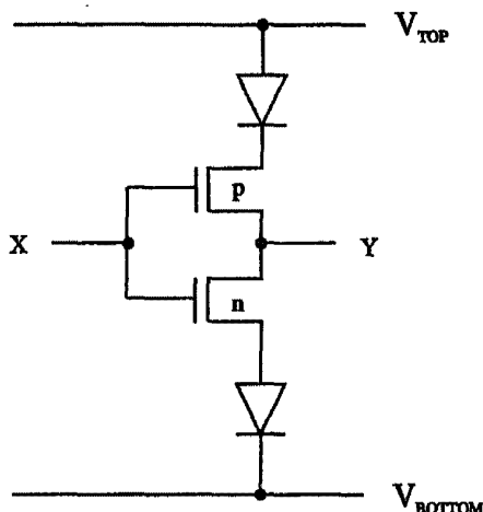
Fig. 7.41 Sample "Hot-Clocking" Circuit
