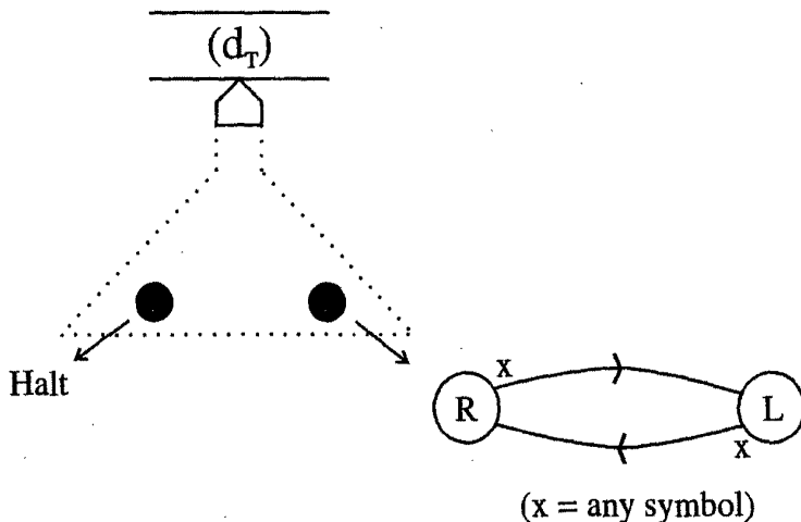
Fig. 3.26 Universal Machine Z
