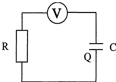
Fig. 7.22 Equivalent RC Circuit
