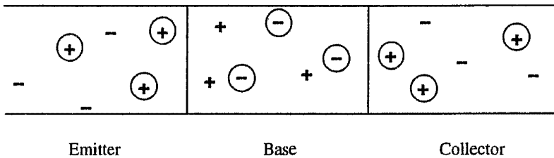
Fig. 7.7 Structure of the npn Bipolar Junction Transistor
