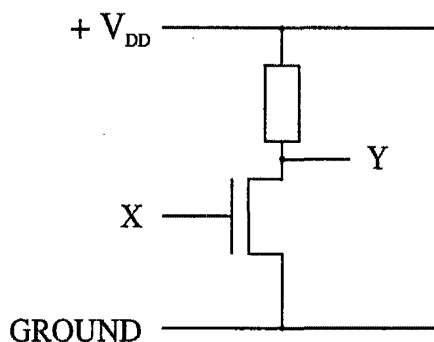
Fig. 7.17 Inverter Circuit
