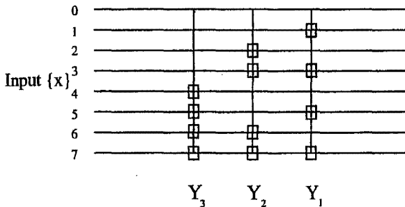
Fig. 2.24 The Three-bit Encoder
