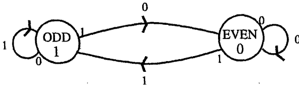
Fig. 3.5 The Parity Machine
