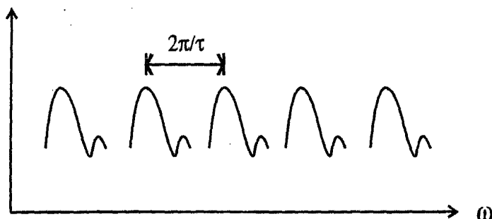
Fig. 4.11 The Fourier Transform of the Sampled Function
