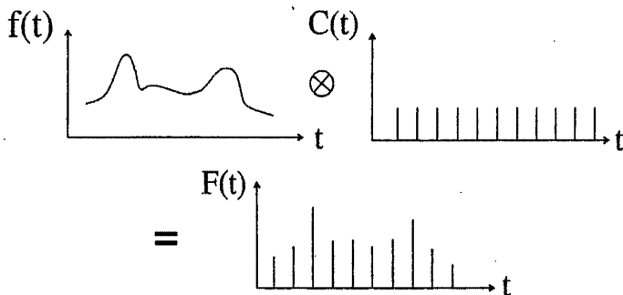
Fig. 4.9 The Sampled Function
