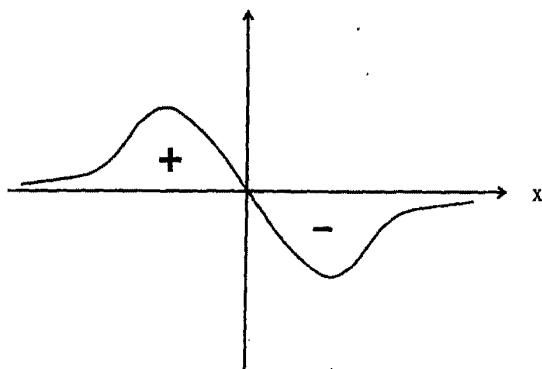
Fig. 7.5 The Net Charge Density
