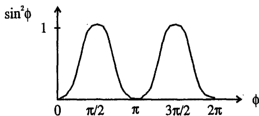
Fig. 5.19 Potential Energy as a function of \phi
