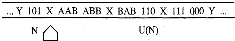
Fig. 3.17 Output Tape from the Locating Machine
