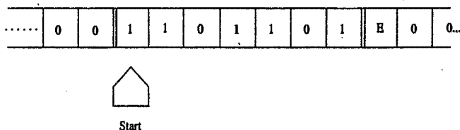
Fig. 3.9 Input Tape for the Parity Counter
