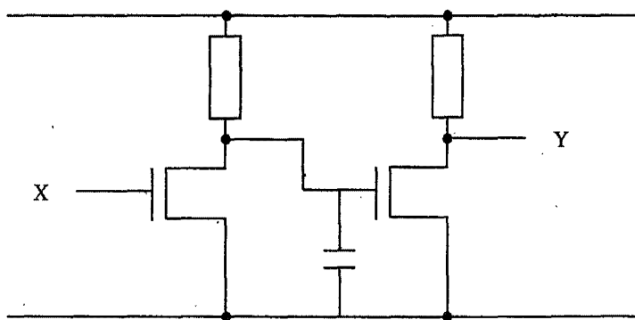
Fig. 7.21 Effective Electrical Analogue of a Follower Circuit
