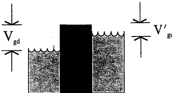
Fig. 7.10 Fluid Analogy for the Back-Biased MOSFET
