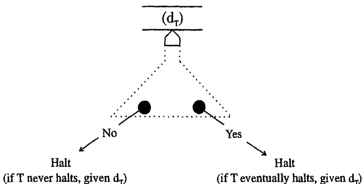
Fig. 3.25 Universal Machine E with input tape d_T
