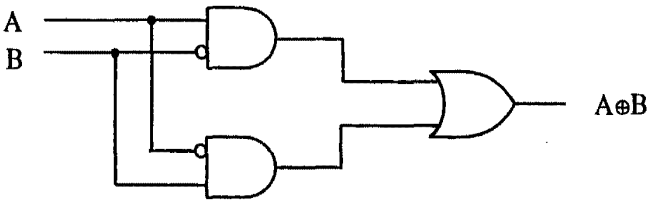
Fig. 2.9 XOR expressed in ANDs and ORs
