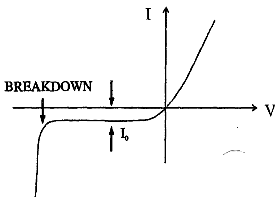
Fig. 7.6 Variation of Diode Current With Voltage
