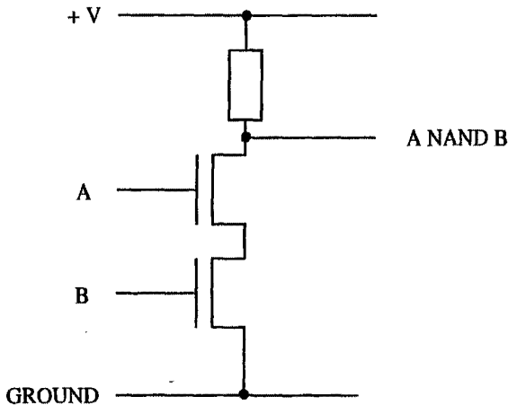
Fig. 2.13 A Transistor NAND Gate
