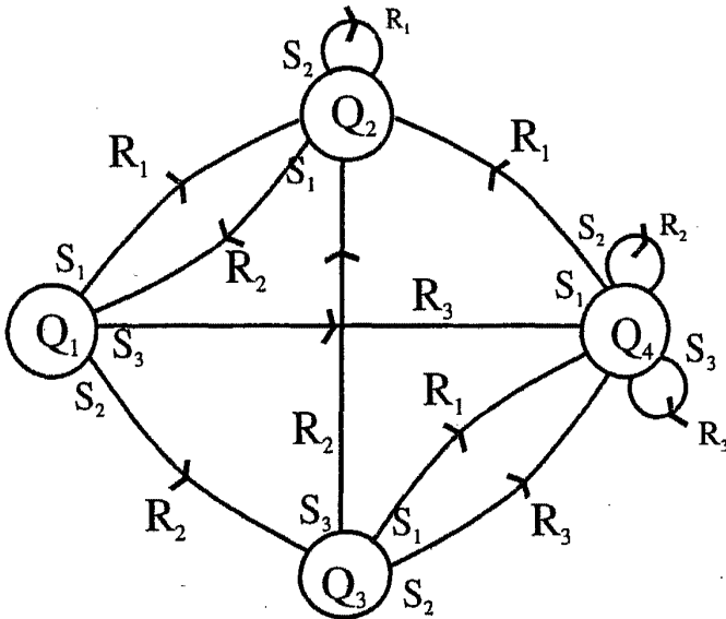
Fig. 3.3 A Complex Finite State Machine
