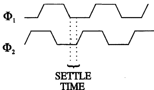
Fig.7.67 The PLA Clock Pulses
