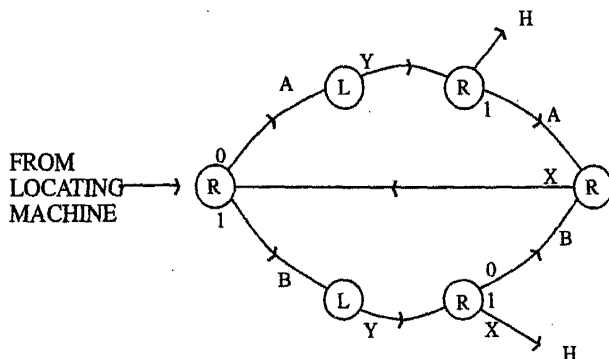
Fig. 3.18 The Copy Machine
