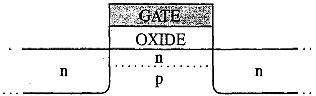
Fig. 7.48 The Depletion Mode Transistor
