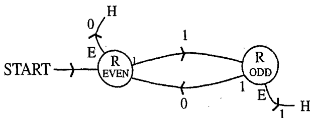
Fig. 3.11 A Turing Machine Parity Counter
