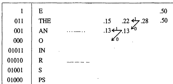
Fig. 4.4 "Trellis" for Huffman Coding
