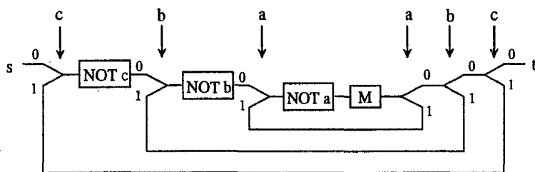
Fig. 6.15 The Operation "Do M Eight Times"
