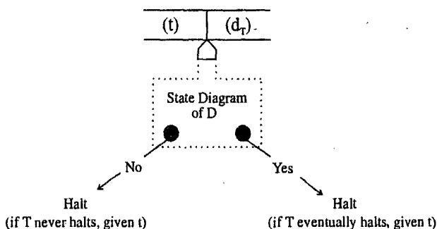
Fig. 3.24 Universal Machine D with tape t and d_T
