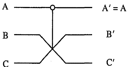
Fig. 5.34 The Fredkin Gate
