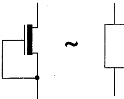
Fig. 7.15 Depletion Mode MOSFET operating as a Resistor
