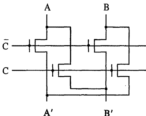
Fig. 7.66 An Exchange Circuit
