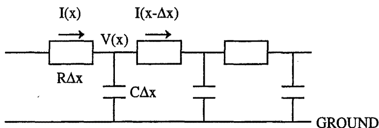
Fig. 7.68 An Infinite-Limit Model of a Simple Wire
