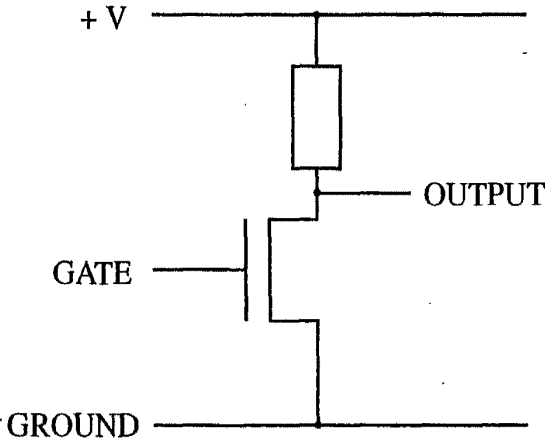
Fig. 2.12 The Transistor Inverter, or NOT Gate
