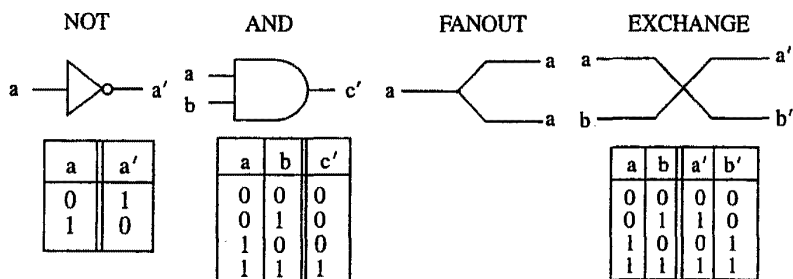
Fig. 6.1 Primitive Elements
