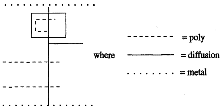
Fig. 7.58 "Stick Figure" for the NAND Gate
