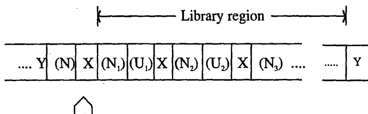
Fig. 3.14 Input Tape to the Locating Machine
