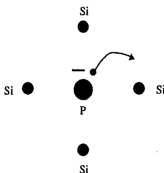
Fig. 7.2 Liberation of a Phosphorus Electron During Doping
