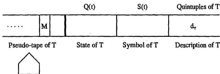
Fig. 3.20 Input Tape to the Universal Turing Machine
