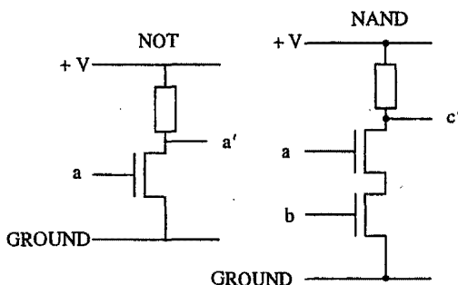
Fig. 6.2 Transistor Circuits for NOT and NAND
