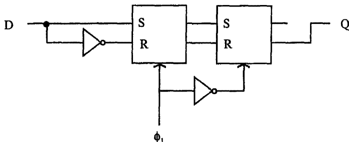
Fig. 2.33 A "D-type" Flip-Flop
