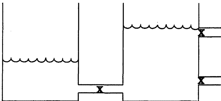
Fig. 7.38 Energy-Saving Analogy for the CMOS Switch
