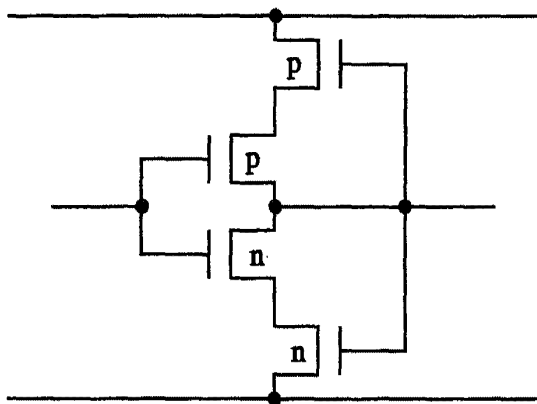
Fig. 7.43 "Diode-less" Hot-Clocking Circuit
