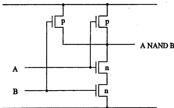
Fig. 7.36 NAND Gate Realized in CMOS
