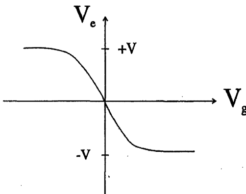
Fig. 7.35 Gate versus Output Voltages for the CMOS Inverter
