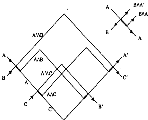
Fig. 5.35 The Fredkin Gate Realized by Billiard Ball Gates
