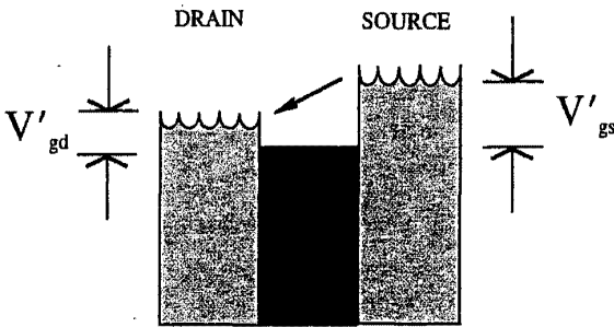
Fig. 7.9 Fluid Analogy for the Forward-Biased MOSFET
