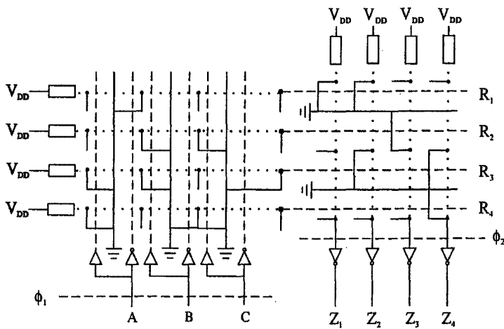
Fig. 7.64 Circuit Diagram for a PLA
