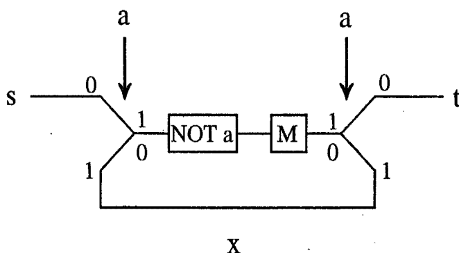
Fig. 6.14 The Operation "Do M Twice"
