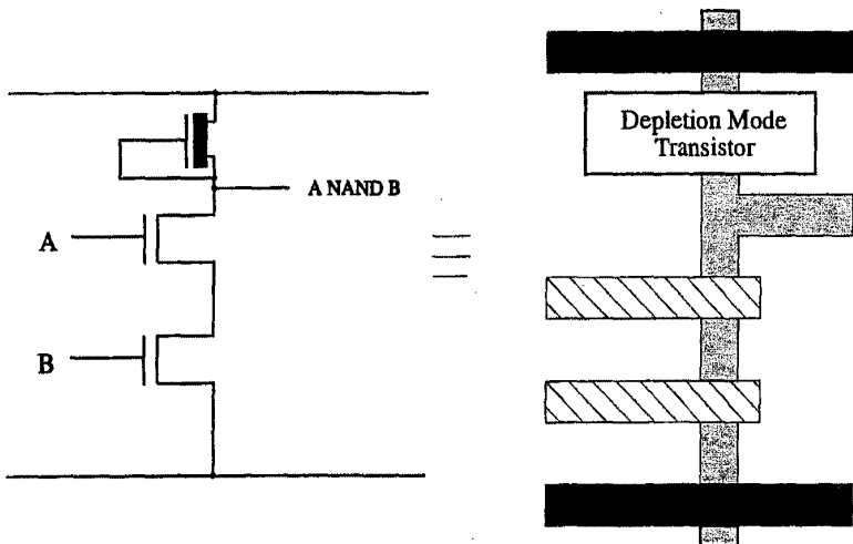
Fig. 7.53 The NAND Gate
