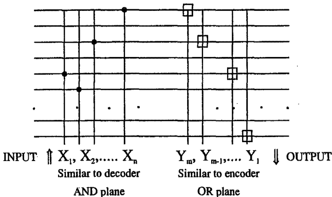
Fig. 2.25 Construction of a General Logical Function
